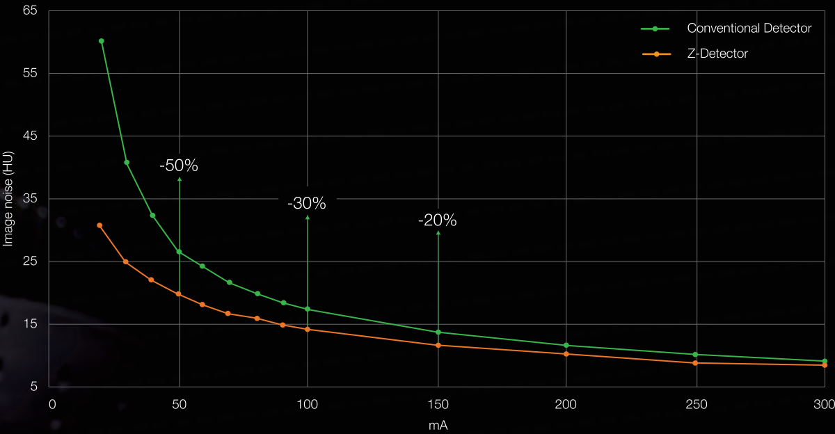
Image noise generated by Z-Detector and the conventional solid-state detector as measured and compared in CT scans using a 180-mm water phantom. The graph illustrates that a reduced noise level is obtained by Z-Detector within the entire range of mAs settings.
